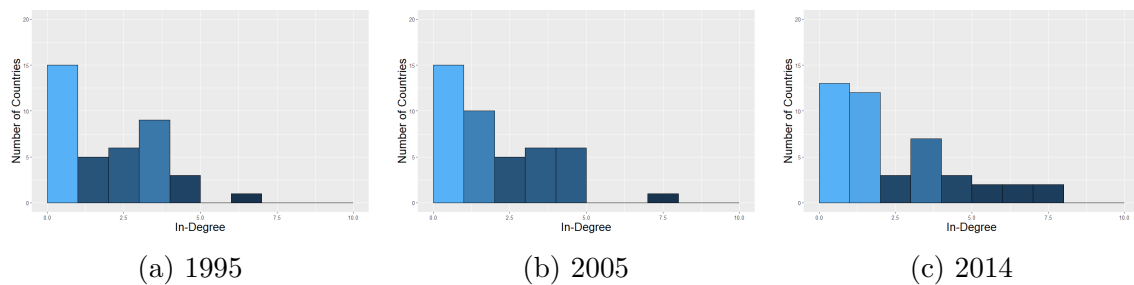
Figure A.5: Distribution of Indegree in the World Trade Network for the years 1995, 2005, and 2014.
