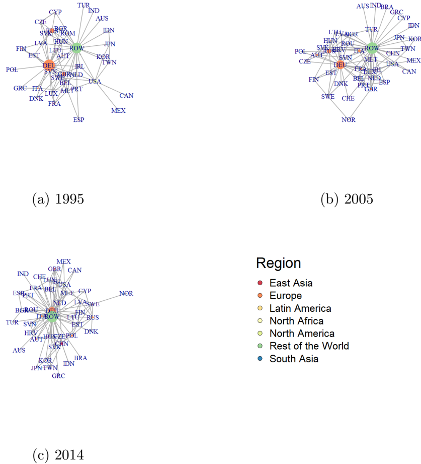
Figure A.10: The World Trade Network with each vertex sized in proportion to their Hub Index for the years 1995, 2005, and 2014.
