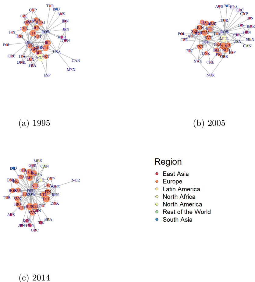
Figure A.12: The World Trade Network with each vertex sized in proportion to their Authority Index for the years 1995, 2005, and 2014.
