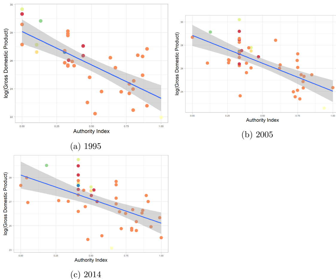
Figure B.9: Correlation between Authority Index in the World Trade Network and Gross Domestic Product for the years 1995, 2005, and 2014.
