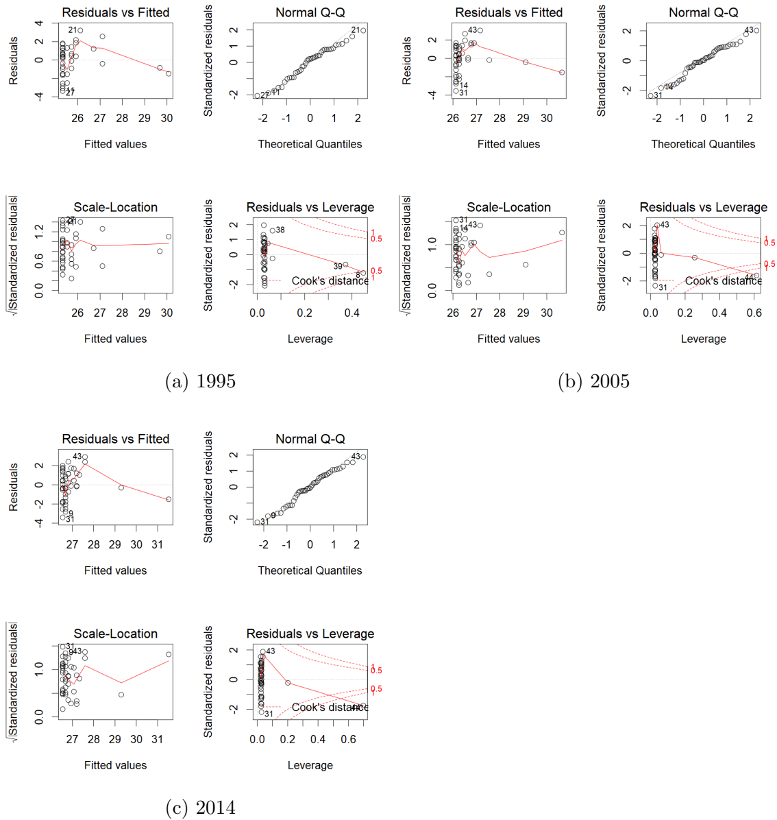
Figure B.4: Regression diagnostics for Outdegree and Gross Domestic Product regression for the years 1995, 2005, and 2014.
