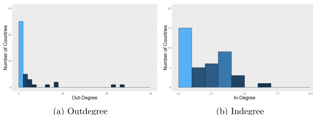
Figure 4.3: Distribution of degree in the World Trade Network in 1995.
