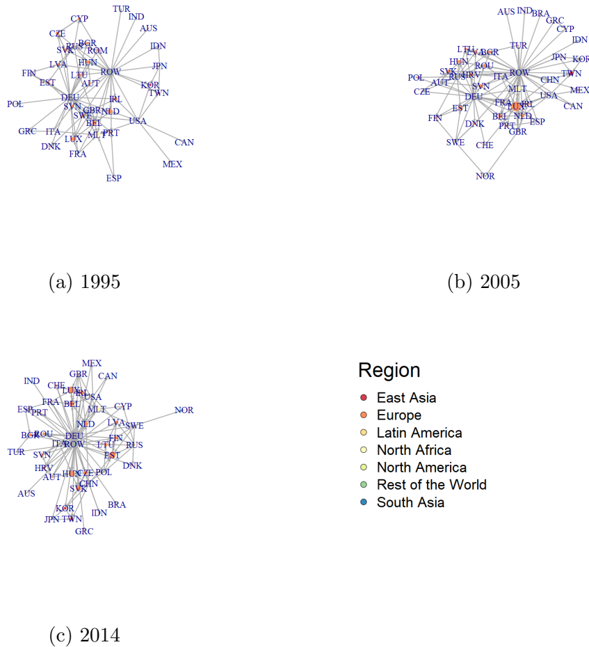
Figure A.4: The World Trade Network with each vertex sized in proportion to Indegree for the years 1995, 2005, and 2014.
