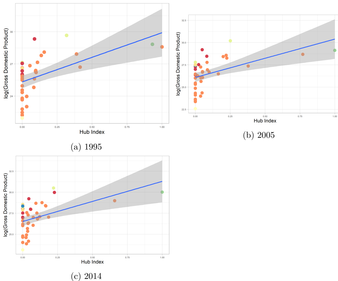
Figure B.7: Correlation between Hub Index in the World Trade Network and Gross Domestic Product for the years 1995, 2005, and 2014.
