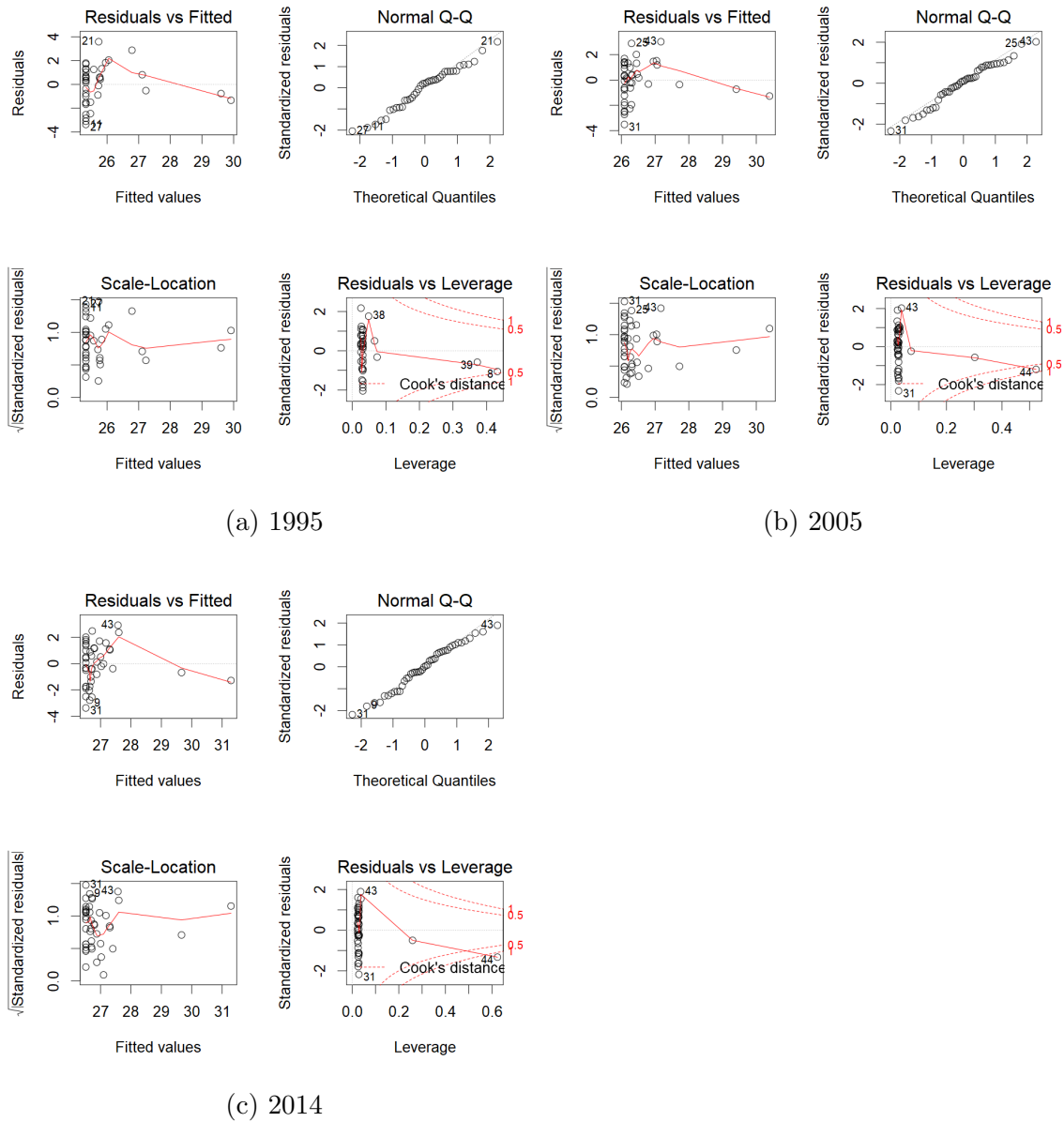
Figure B.8: Regression diagnostics for Hub Index and Gross Domestic Product regression for the years 1995, 2005, and 2014.
