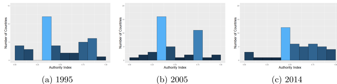
Figure A.13: Distribution of countries' Authority Index in the World Trade Network for the years 1995, 2005, and 2014.
