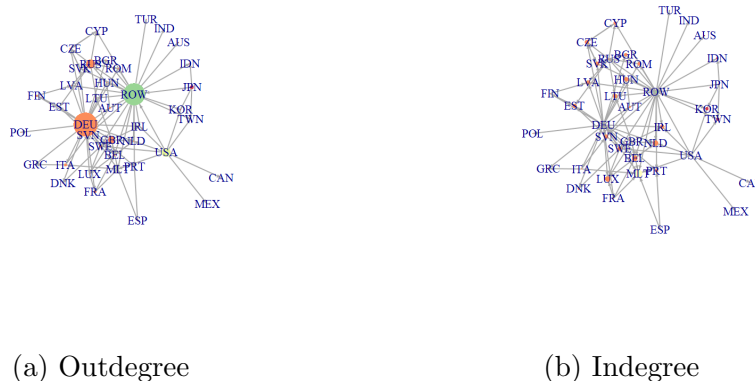
Figure 4.2: The World Trade Network sized in proportion to indegree and outdegree in 1995.
