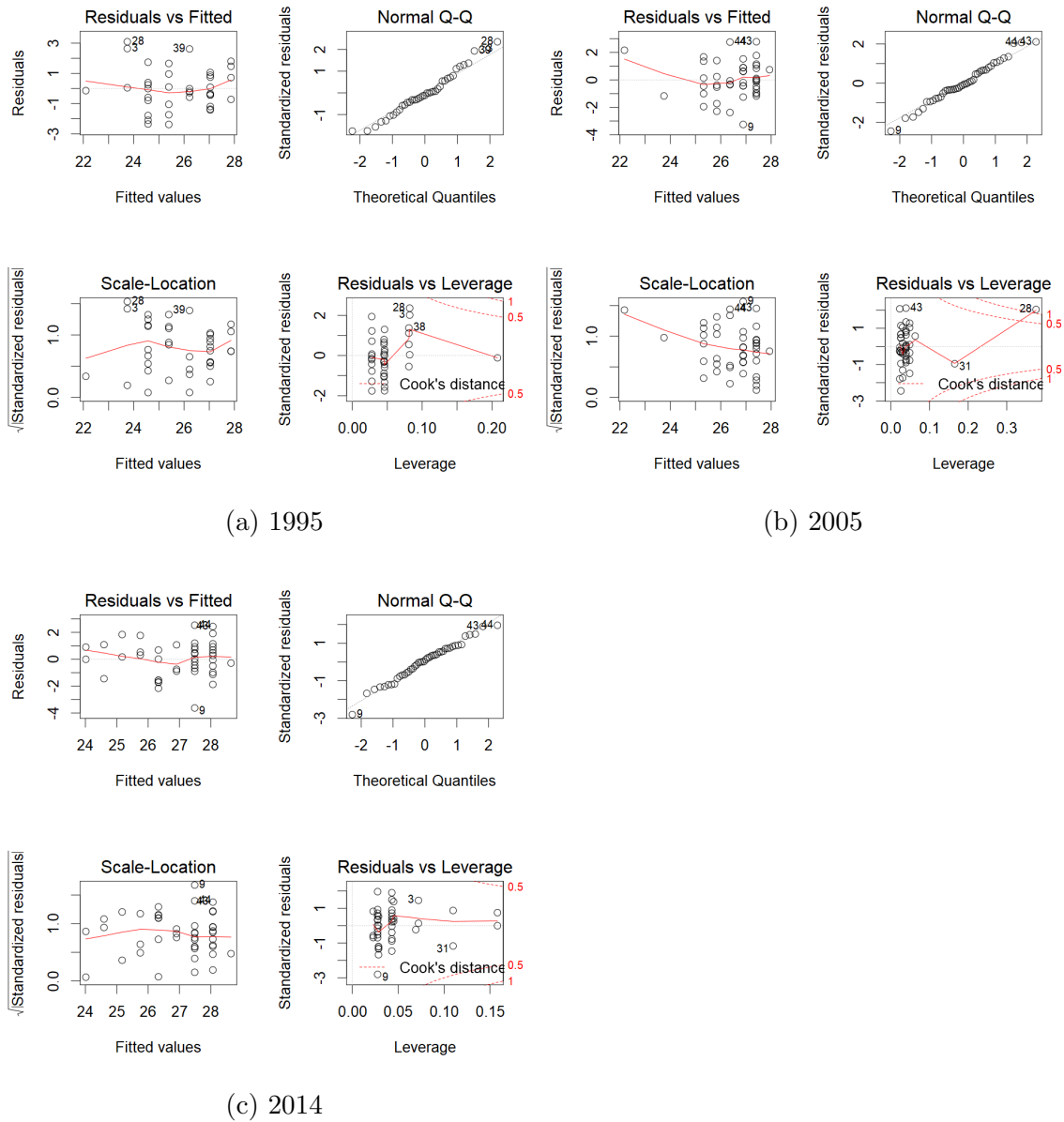
Figure B.2: Regression diagnostics for Indegree and Gross Domestic Product regression for the years 1995, 2005, and 2014.
