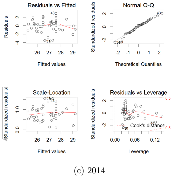
Figure B.10: Regression diagnostics for Authority Index and Gross Domestic Product regression for the years 1995, 2005, and 2014.
