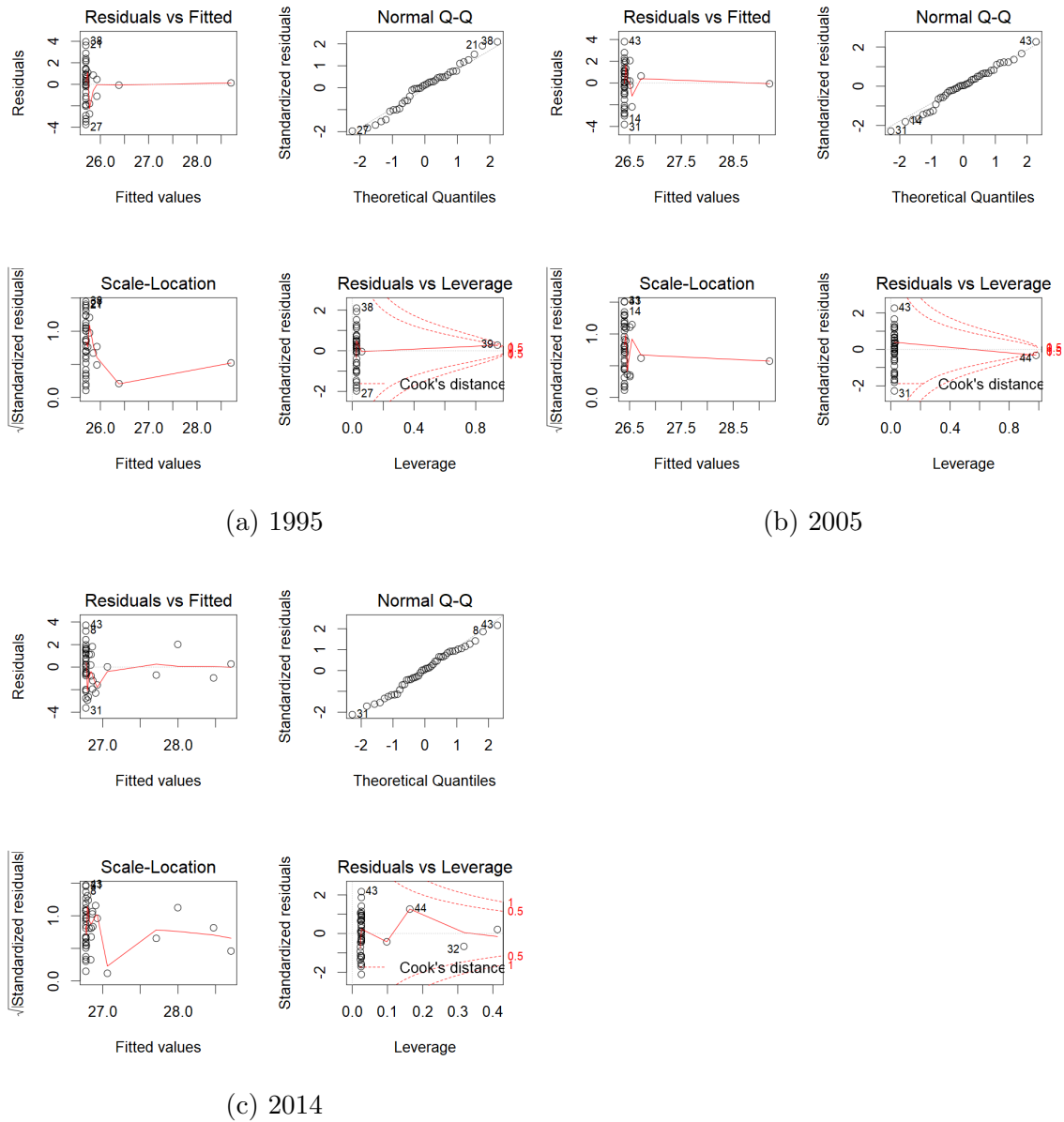
Figure B.6: Regression diagnostics for Betweenness and Gross Domestic Product regression for the years 1995, 2005, and 2014.
