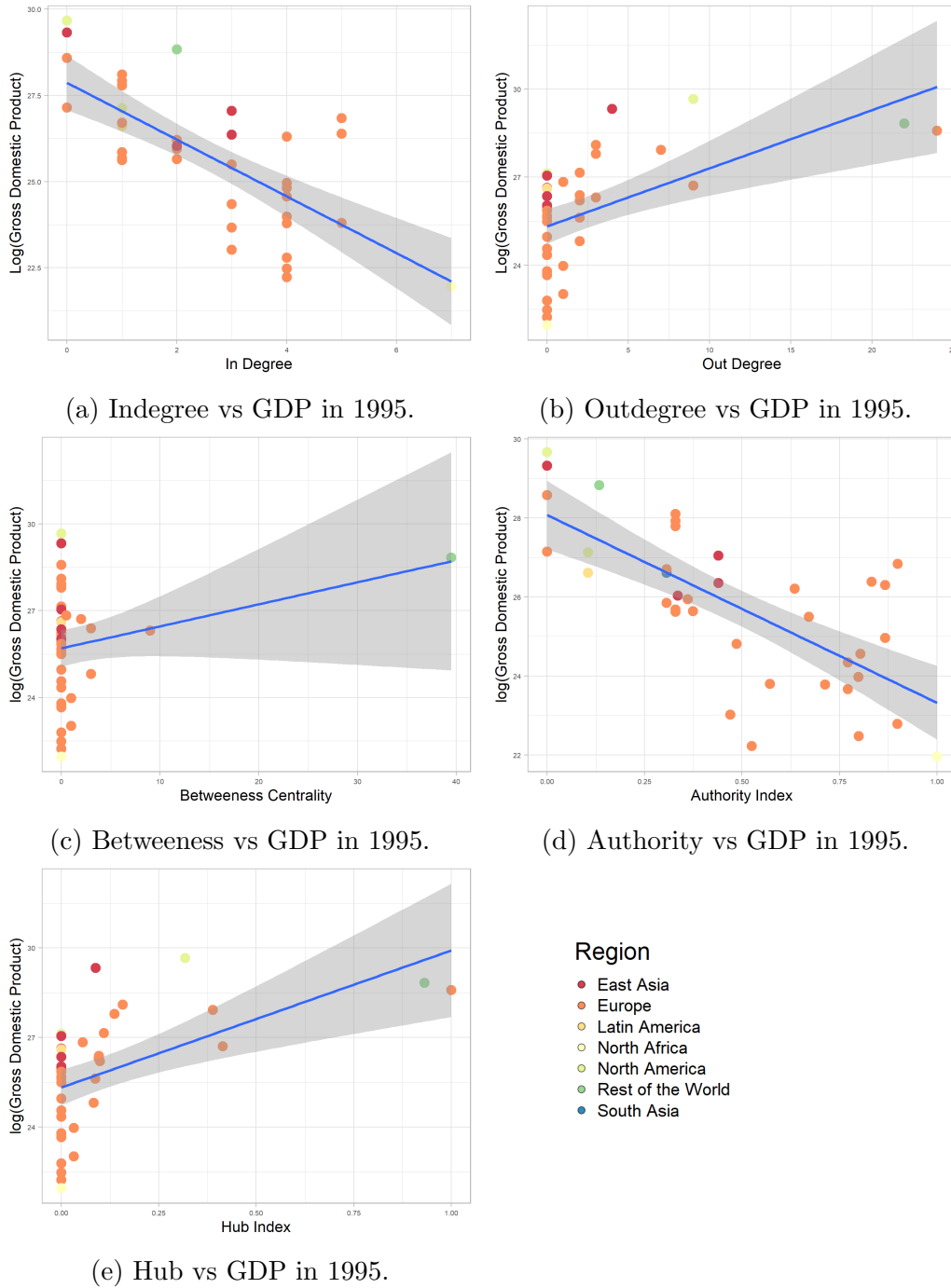
Figure 4.7: Regression between network measures and Gross Domestic Product in the World Trade Network in 1995.
