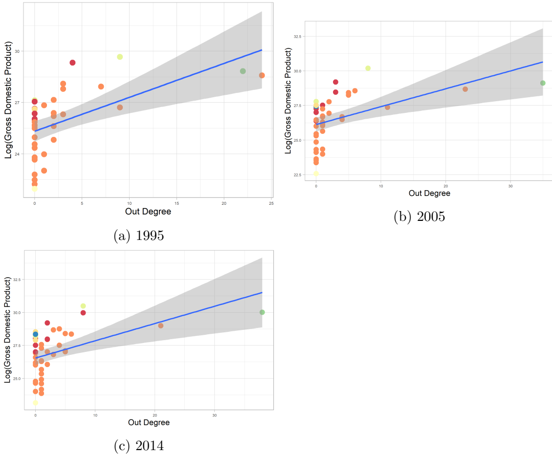
Figure B.3: Correlation between Outdegree in the World Trade Network and Gross Domestic Product for the years 1995, 2005, and 2014.
