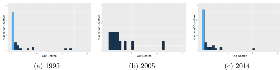
Figure A.7: Distribution of Outdegree in the World Trade Network for the years 1995, 2005, and 2014.
