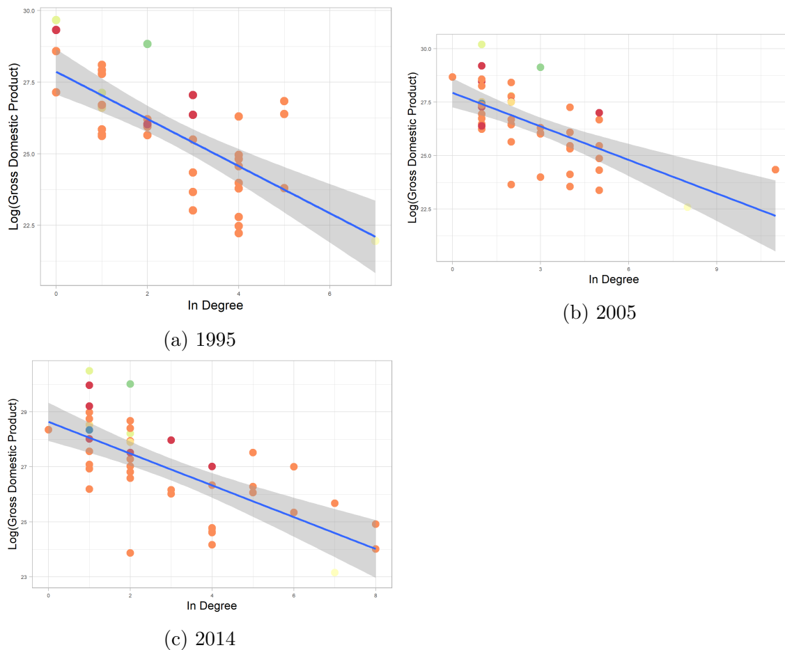
Figure B.1: Correlation between Indegree in the World Trade Network and Gross Domestic Product for the years 1995, 2005, and 2014.
