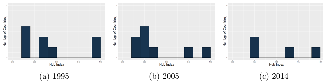
Figure A.11: Distribution of countries' Hub Index in the World Trade Network for the years 1995, 2005, and 2014.
