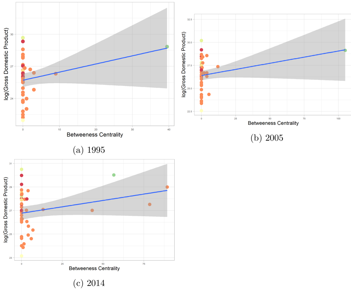
Figure B.5: Correlation between Betweenness in the World Trade Network and Gross Domestic Product for the years 1995, 2005, and 2014.
